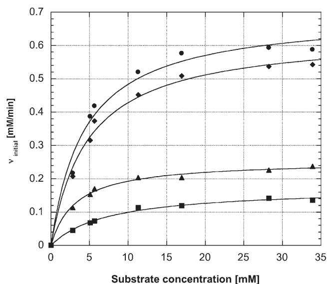
Figure 1. Saturation kinetics plots for the reduction of N -acetamidoacrylic acid with [\text{Rh}(\text{COD})\text{Biot-1}]^+ (9% DMSO, measured: squares), [\text{Rh}(\text{COD})\text{Biot-1}]^+ \subset WT Sav (9% DMSO, measured: triangles), [\text{Rh}(\text{COD})\text{Biot-(R)-Pro-1}]^+ \subset WT Sav (30% DMSO, measured: circles) and [\text{Rh}(\text{COD})\text{Biot-(R)-Pro-1}]^+ \subset WT Avi (30% DMSO, measured: diamonds). All the fitted graphics are shown in solid lines.
