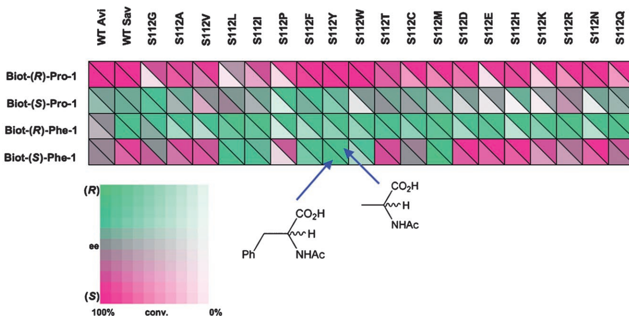
Scheme 3. Fingerprint display of the results of the chemogenetic optimization for the reduction of \alpha -acetamidoacrylic acid (top triangle) and \alpha -acetamidocinnamic acid (bottom triangle).
