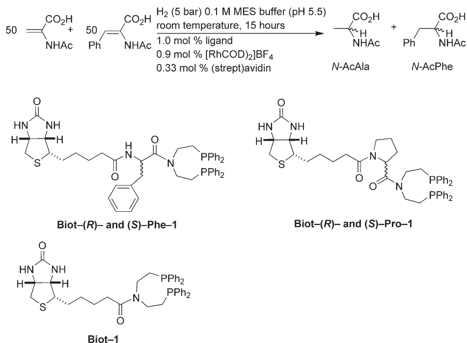
Scheme 2. Biotinylated ligands used in this study and standard operating conditions for the hydrogenation of a cocktail mixture containing \alpha -acetamidoacrylic acid and \alpha -acetamidocinnamic acid (50 equivalents of each with respect to the biotinylated ligand).
